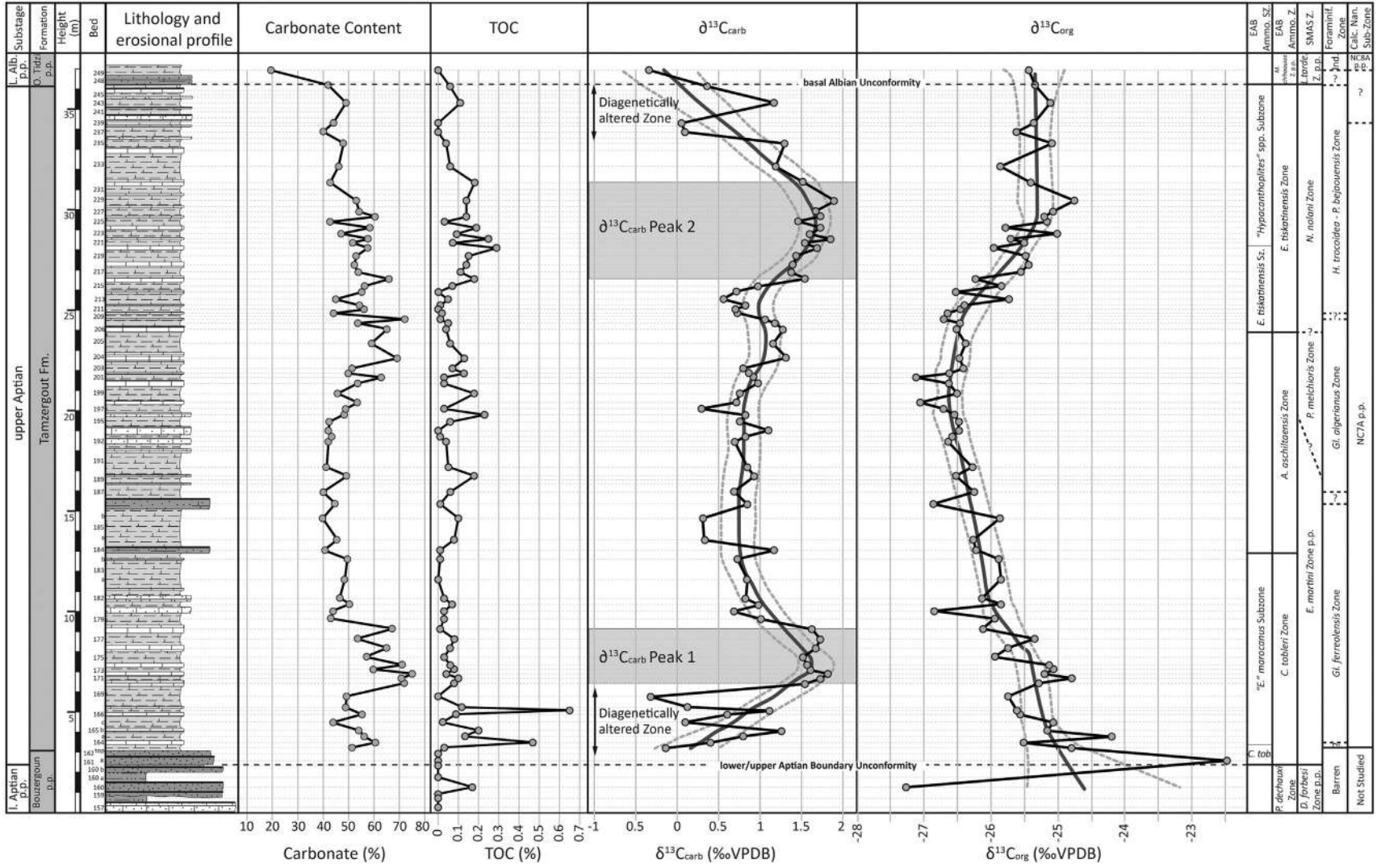
Fig. 14. Carbonate content, total organic carbon (TOC), \delta^{13}C_{carb} and \delta^{13}C_{org} (% VDPB) of the Lower Aptian to Lower Albian at Tiskatine, EAB. Findings are referenced against the local ammonoid zonation scheme in the EAB of Luber et al. (2017) , the Standard Mediterranean Ammonite Scale (SMAS) of Reboulet et al. (2011, 2014) , standard planktonic foraminiferal zonation of Premoli Silva and Verga (2004) and Lower Cretaceous NC Zones of Roth (1978, 1983) and subzones after Bralower et al. (1993) .
