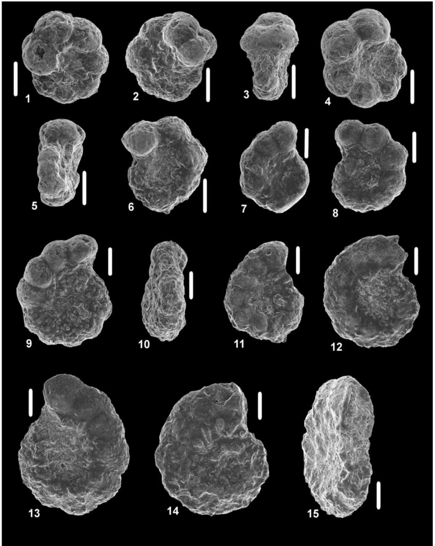
Fig. 8. Plate 1: Scanning electron microscope images of selected planktonic foraminifera from the Tiskatine section, Morocco (all scale bars = 0.1 mm): (1–3) Globigerinelloides barri (Bolli, Loeblich and Tappan, 1957) from MTTK 197 ; (4–6) Globigerinelloides ferreolensis (Bolli, Loeblich and Tappan, 1957) from MTTK 197 ; (7–8) G. ferreolensis - G. algerianus transitional form from MTTK 185a ; (9–11) Globigerinelloides algerianus Cushman and Ten Dam, 1948 from MTTK 197 ; (12–13) Pseudoplanomalina cheniourensis (Sigal, 1952) from MTTK 217 ; (14–15) Pseudoplanomalina cheniourensis (Sigal, 1952) from MTTK 237 .
