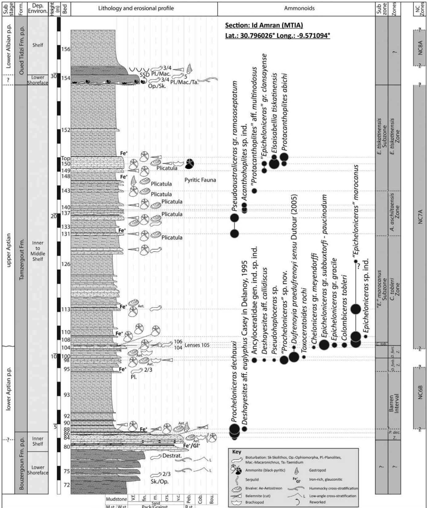
Fig. 4. Id Amran section. Distribution of ammonoids, key calcareous nanofossils, and biostratigraphic interpretation. Distribution charts for calcareous nanofossil can be found in the supplementary data.
